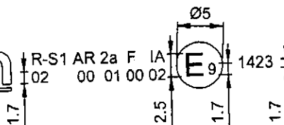
Prüfnummer/ layout of approval marking
