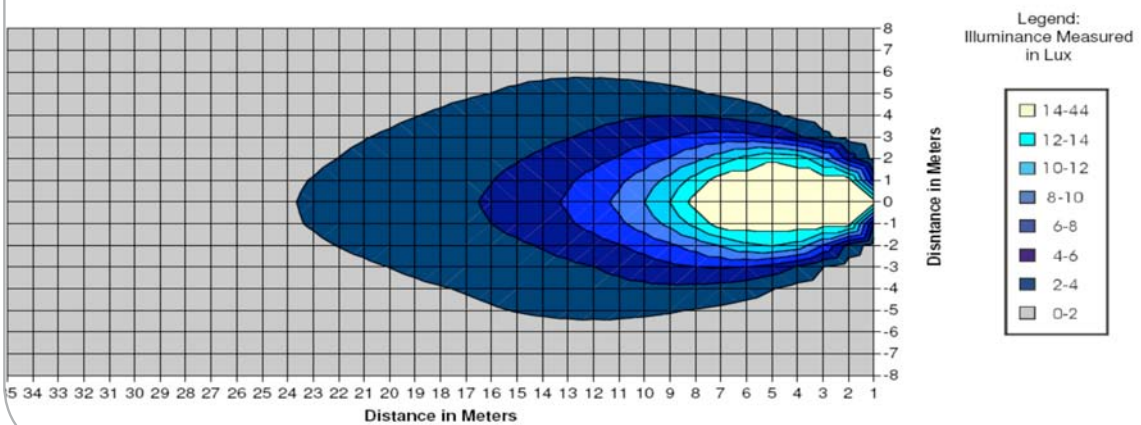
81263 - LED Medium Flood Lamp Bird's Eye View Plot 26-Aug-08 Tested By: C. Aubert
