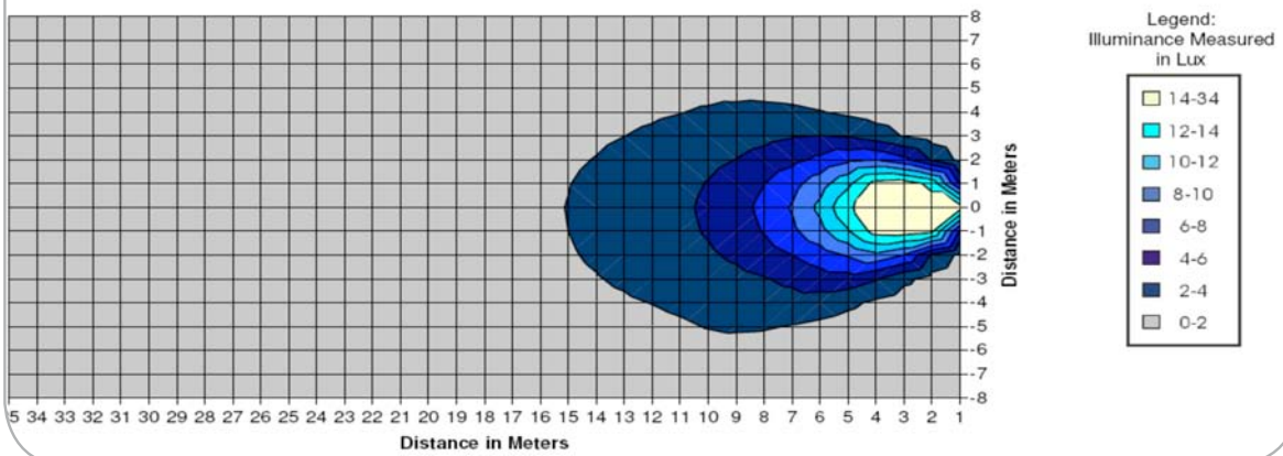
81262 - LED Wide Flood Bird's Eye View Plot 26-Aug-08 Tested By: C. Aubert
