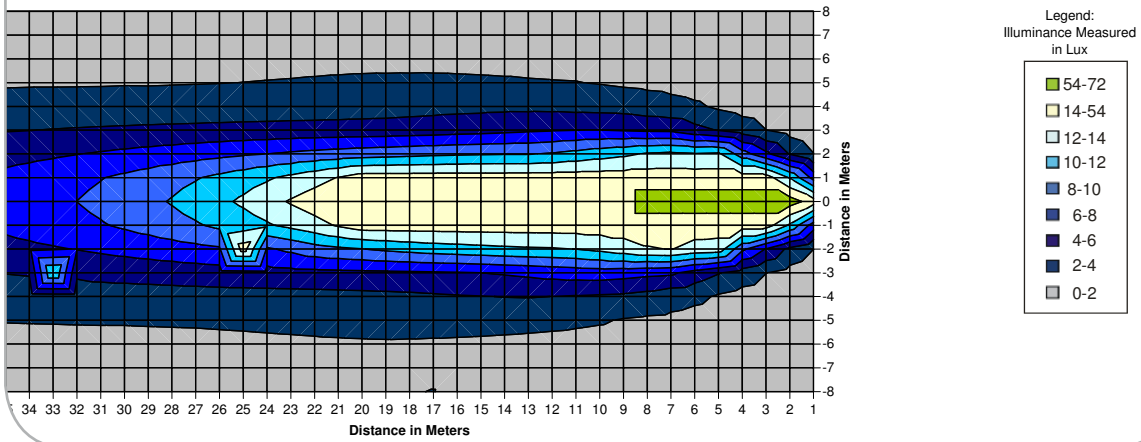
81261/HO High Output LED Spot Lamp Bird's Eye View Plot 10-Dec-08 Tested By: C. Aubert
